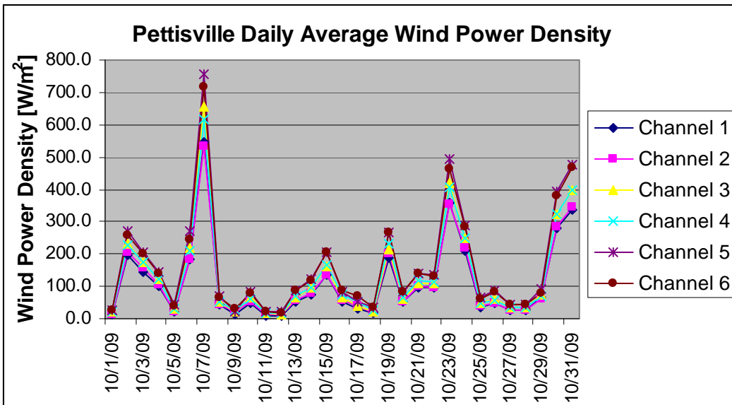
Figure 4: Pettisville Daily Average Wind Power Density for October 2009
