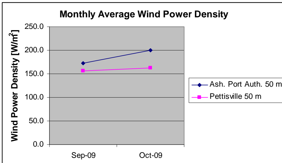
Figure 4: Monthly Average Wind Power Density
