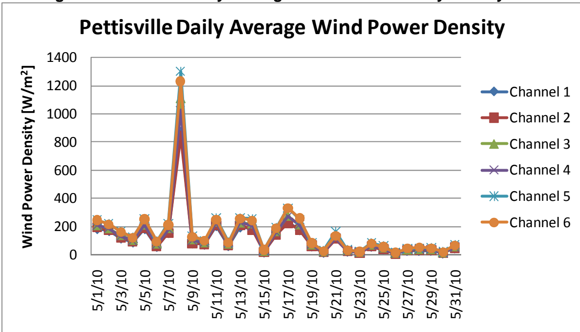
Figure 4: Pettisville Daily Average Wind Power Density for May 2010
