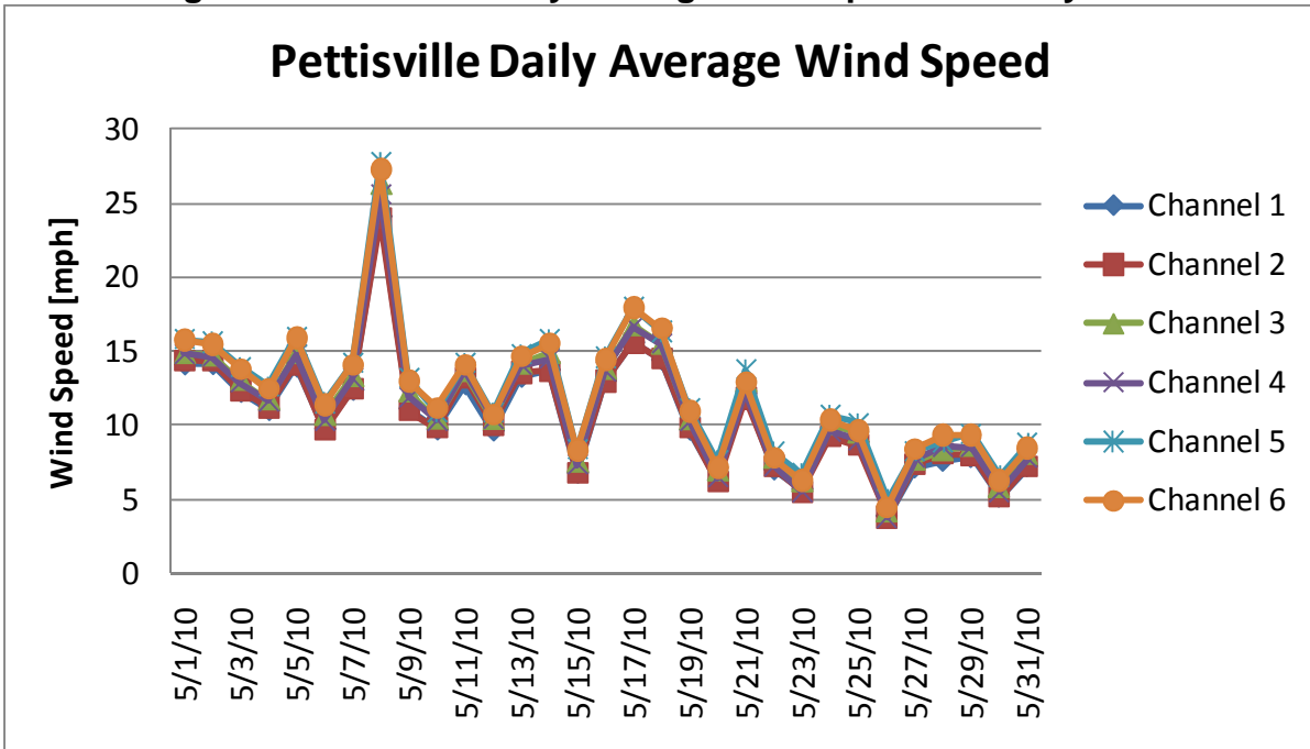
Figure 3: Pettisville Daily Average Wind Speeds for May 2010
