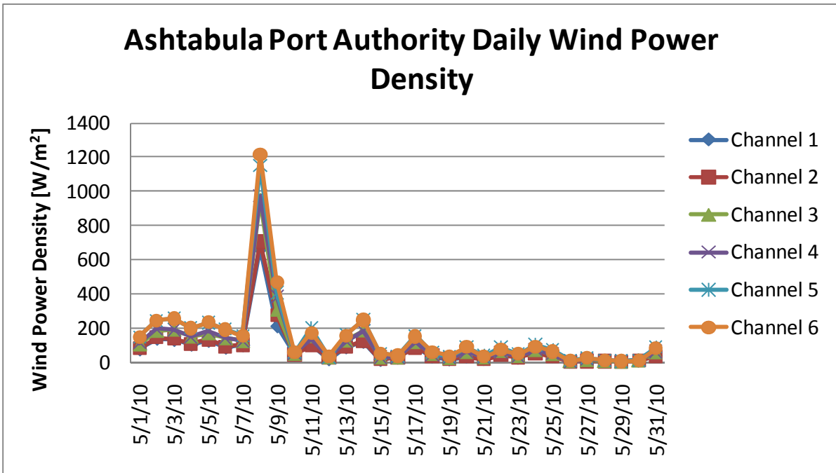
Figure 2: Ashtabula Port Authority Daily Average Wind Power Density for May 2010
