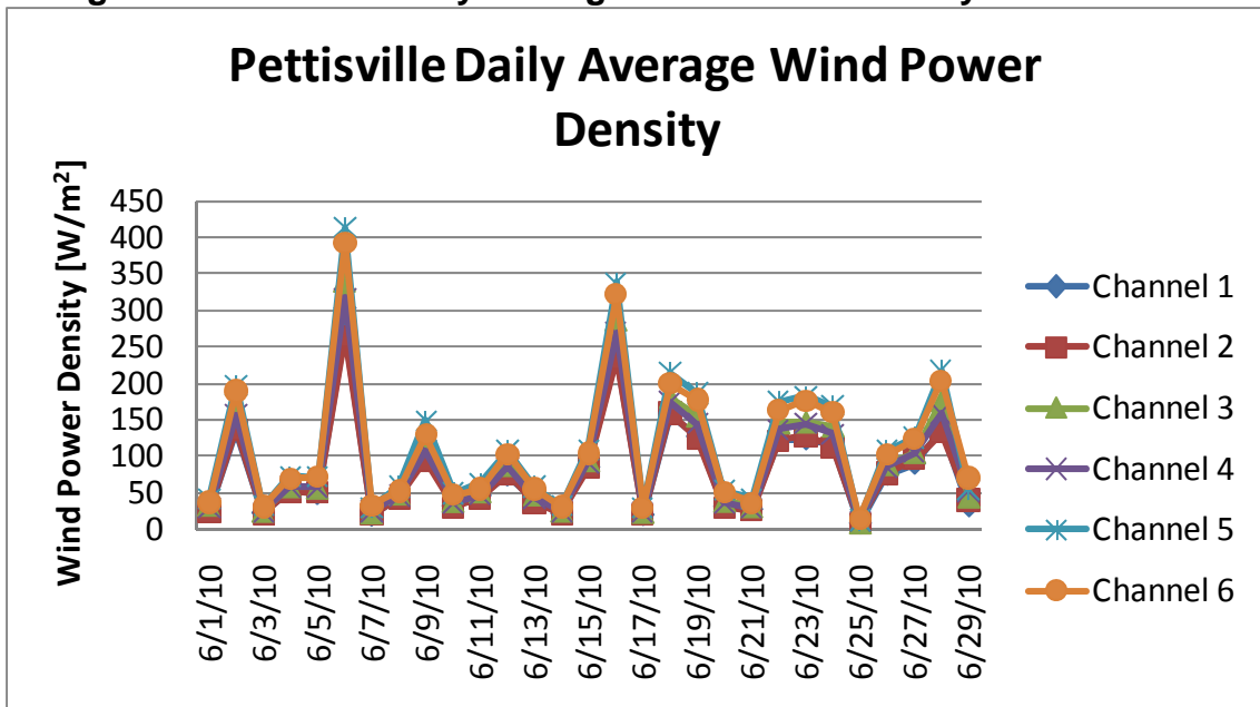
Figure 4: Pettisville Daily Average Wind Power Density for June 2010
