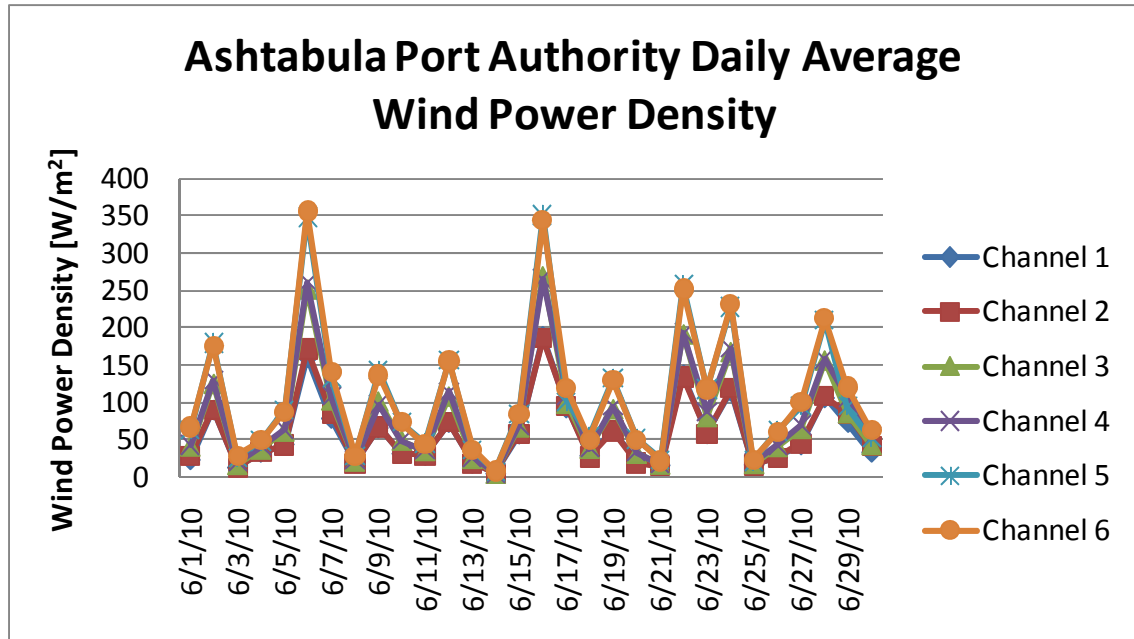
Figure 2: Ashtabula Port Authority Daily Average Wind Power Density for June 2010
