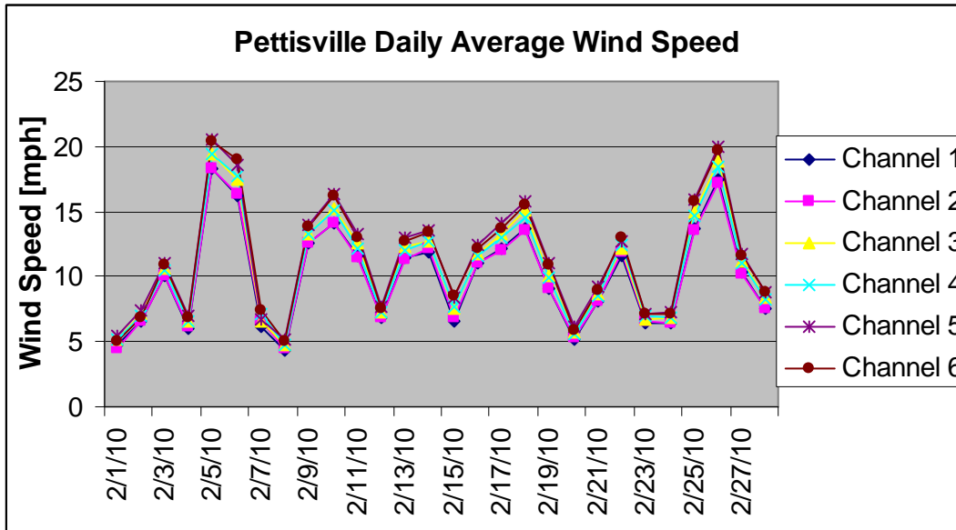
Figure 3: Pettisville Daily Average Wind Speeds for February 2010
