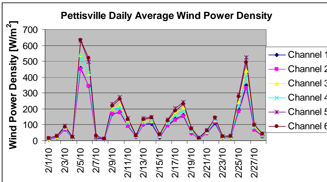
Figure 4: Pettisville Daily Average Wind Power Density for February 2010
