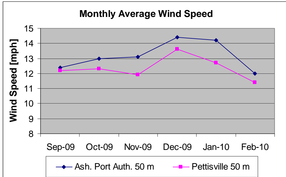
Figure 5: Monthly Average Wind Speeds (Data Filtered for Icing and Tower Shading)
