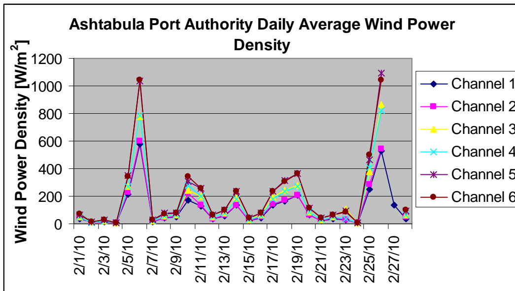
Figure 2: Ashtabula Port Authority Daily Average Wind Power Density for February 2010
