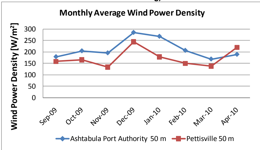
Figure 6: Monthly Average Wind Power Density (Data Filtered for Icing and Tower Shading)
