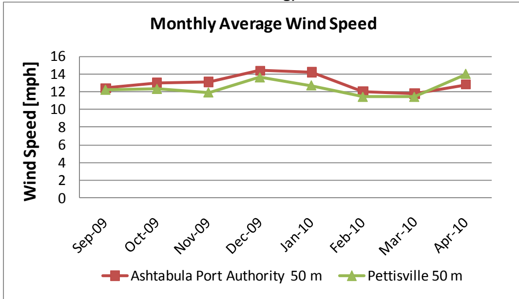
Figure 5: Monthly Average Wind Speeds (Data Filtered for Icing and Tower Shading)
