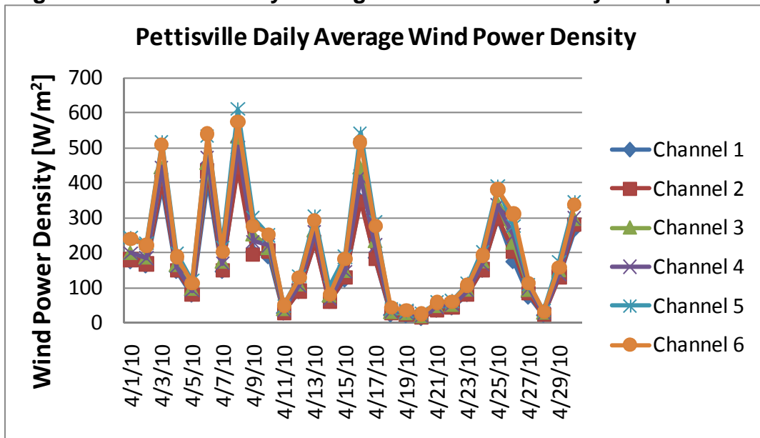
Figure 4: Pettisville Daily Average Wind Power Density for April 2010
