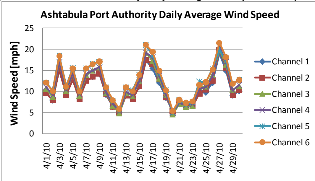
Figure 1: Ashtabula Port Authority Daily Average Wind Speeds for April 2010
