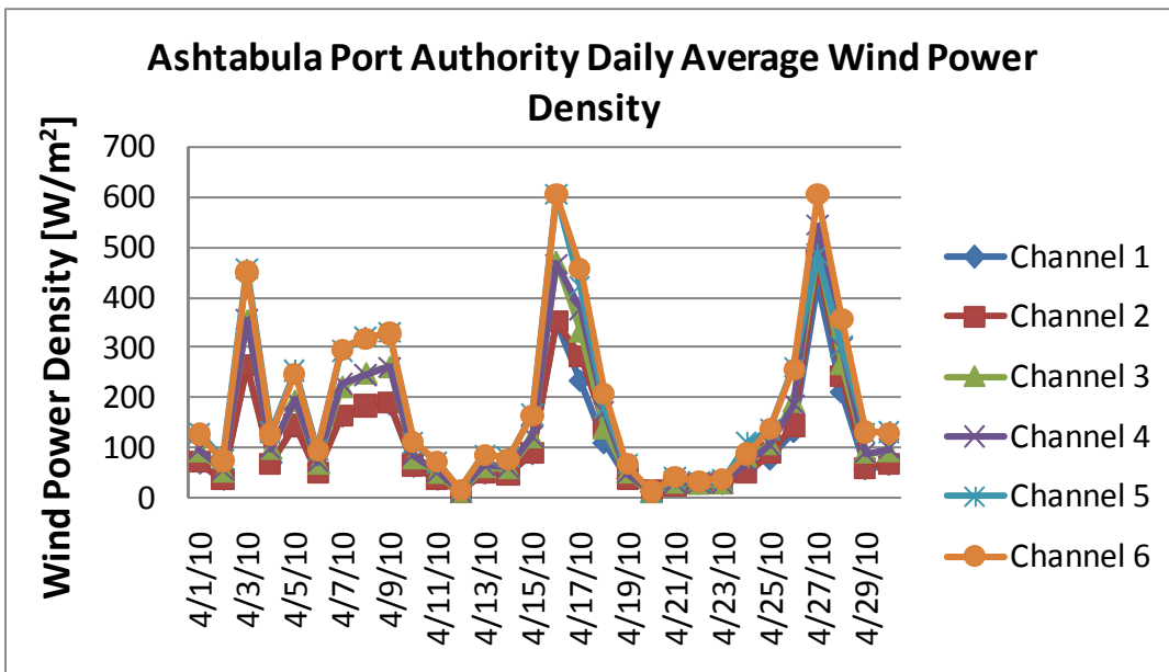
Figure 2: Ashtabula Port Authority Daily Average Wind Power Density for April 2010
